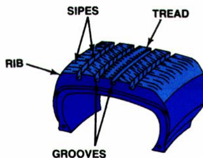
TIRE TREAD
