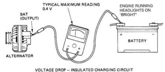
VOLTAGE DROP – INSULATED CHARGING CIRCUIT
