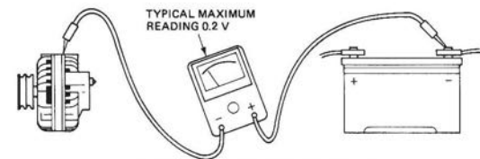
VOLTAGE DROP – GROUND CHARGING CIRCUIT
