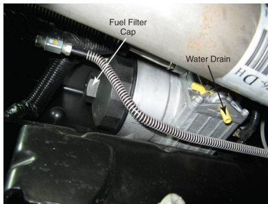
FIGURE 7-3 A fuel heater is part of the fuel filter and water separator located on the frame rail of a Ford pickup truck equipped with a PowerStroke 6.0 liter V-8 diesel engine.
