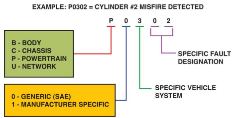
FIGURE 11-2 OBD-II DTC identification format.
