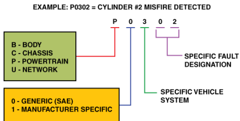
Figure 10.2 OBD-II DTC identification format.
