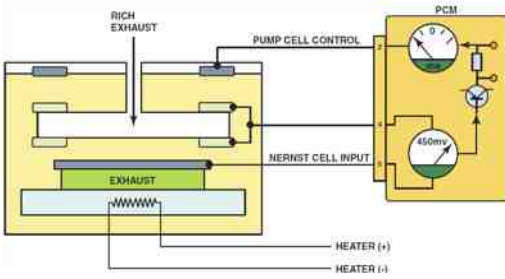
FIGURE 25-7 When the exhaust is rich, the PCM applies a negative current into the pump cell.
