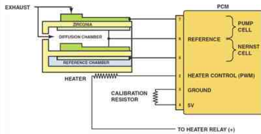
FIGURE 25-6 The reference electrodes are shared by the Nernst cell and the pump cell.
