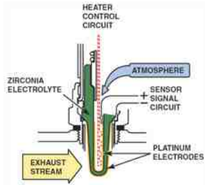
FIGURE 25-4 A typical heated zirconia oxygen sensor, showing the sensor signal circuit that uses the outer (exhaust) electrode as negative and the ambient air side electrode as the positive.
