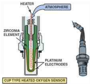
FIGURE 25-3 Most conventional zirconia oxygen sensors and some wide-band oxygen sensors use the cup-type design.
