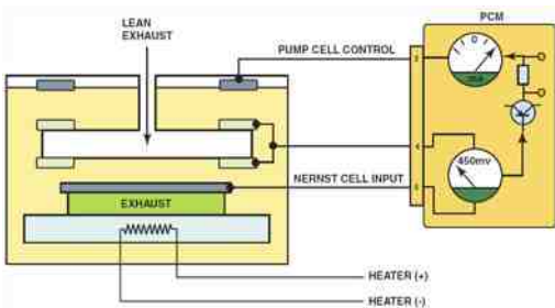
FIGURE 25-8 When the exhaust is lean, the PCM applies a positive current into the pump cell.
