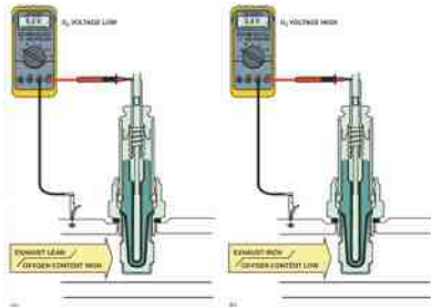
FIGURE 25-2 (a) When the exhaust is lean, the output of a zirconia oxygen sensor is below 450 mV. (b) When the exhaust is rich, the output of a zirconia oxygen sensor is above 450 mV.
