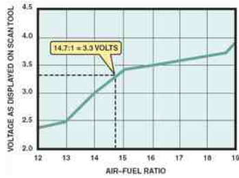
FIGURE 25-11 The scan tool can display various voltage but will often show 3.3 volts because the PCM is controlling the sensor by applying a low current to the sensor to achieve balance.
