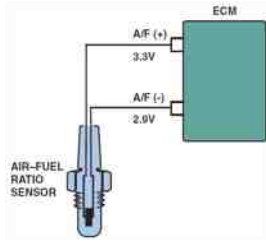
FIGURE 25-10 A single cell wide-band oxygen sensor has four wires with two for the heater and two for the sensor itself. The voltage applied to the sensor is 0.4 volt (3.3 - 2.9 = 0.4) across the two leads of the sensor.
